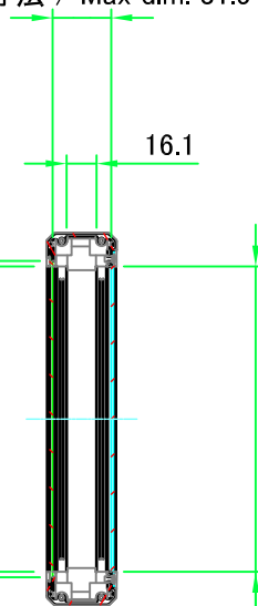
ねじ止めパネル有効寸法 / Screwed panel Max dim. D-36
